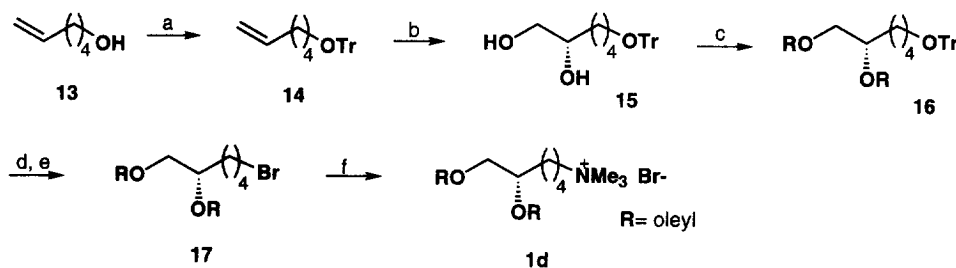
Scheme 3. Reagents and conditions: (a) TrCl (1.2 equiv), Py, 60 °C, 3 h, 89%; (b) AD-mix- \alpha , t -BuOH-H 2 O, 0 °C, 36 h, 90%; (c) RI (3 equiv), NaH (2.5 equiv), DMF, 80 °C, 4 h, 19%; (d) THF-2 N HCl, reflux, 1 h, 92%; (e) CBr 4 (1.5 equiv), Ph 3 P (1.5 equiv), CH 2 Cl 2 , rt, 4 h, 87%; (f) Me 3 N-DMSO, rt, 72 h, pressure tube, 55%.
